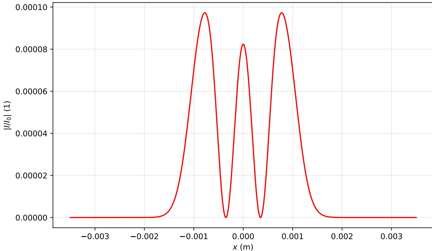
Intensity profile I(x, y = 0, z = 0.159)/I_0 , P_{in}=8.0P_{cr} , artificial time
